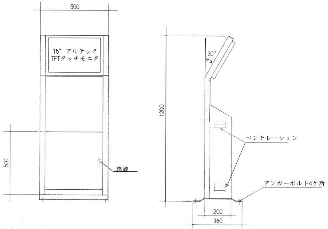
[外形寸法図<mm>]
